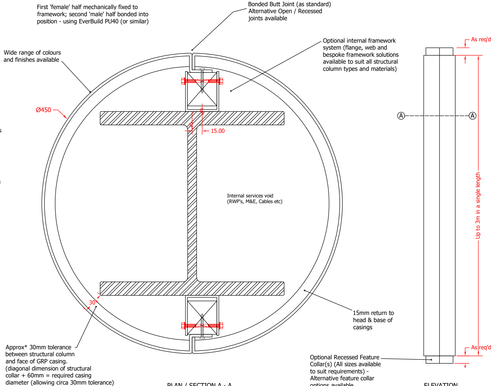
PLAN / SECTION A - A
