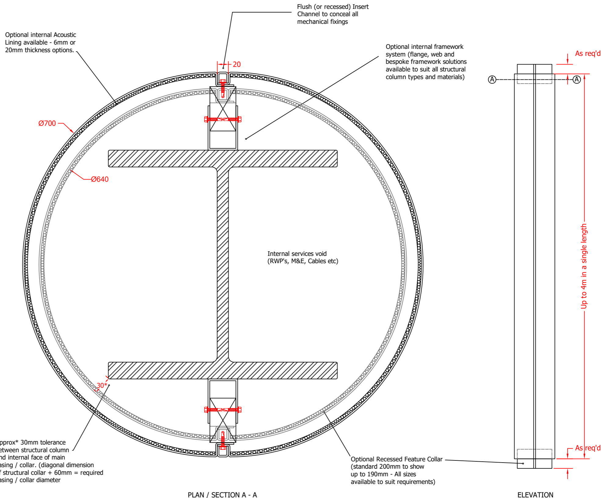
PLAN / SECTION A - A
