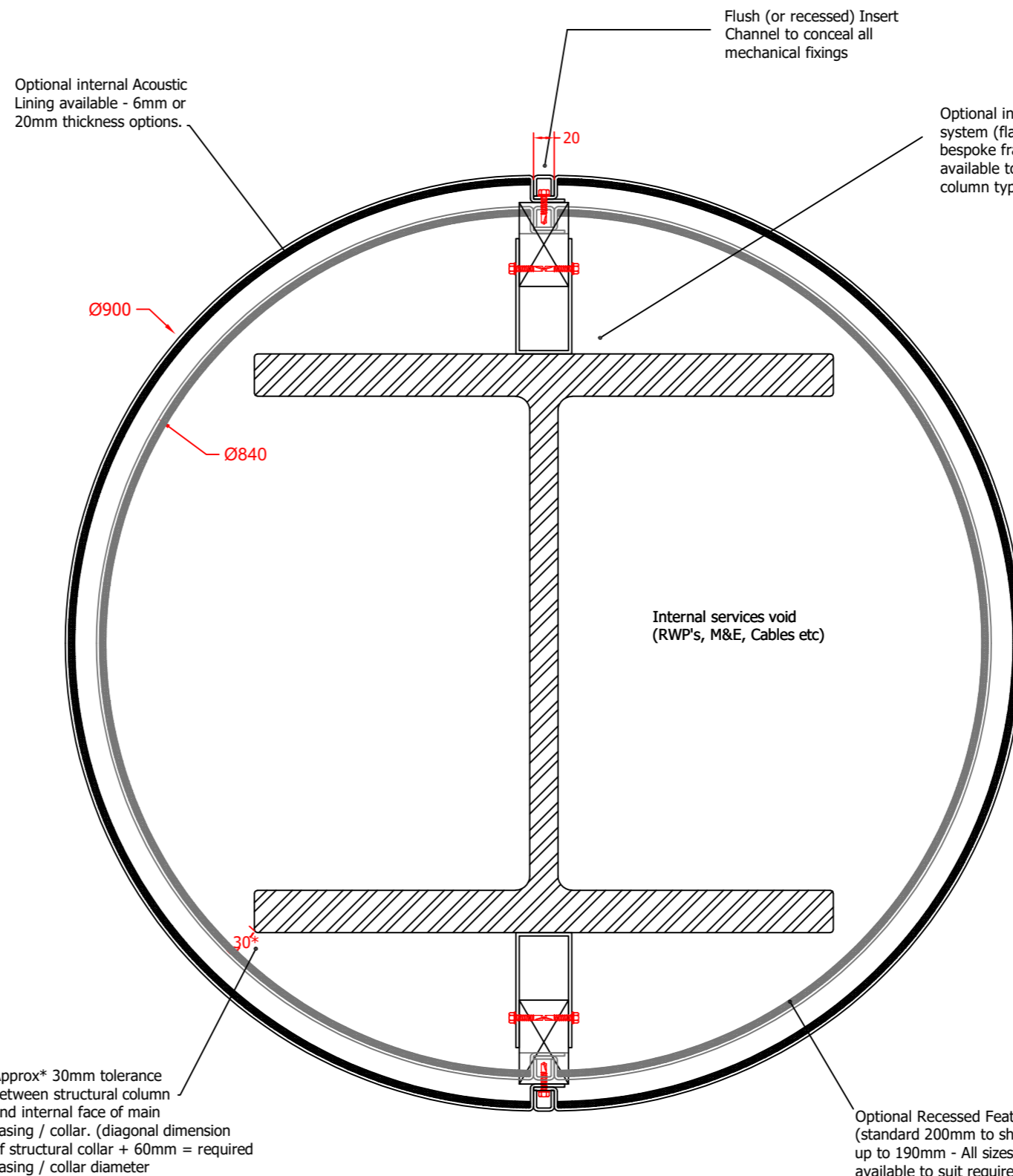
PLAN / SECTION A - A
