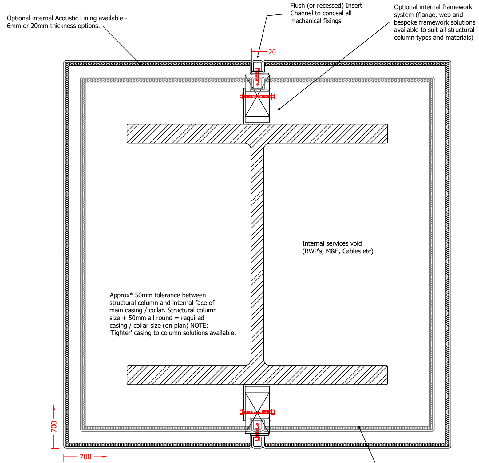
PLAN / SECTION A - A
