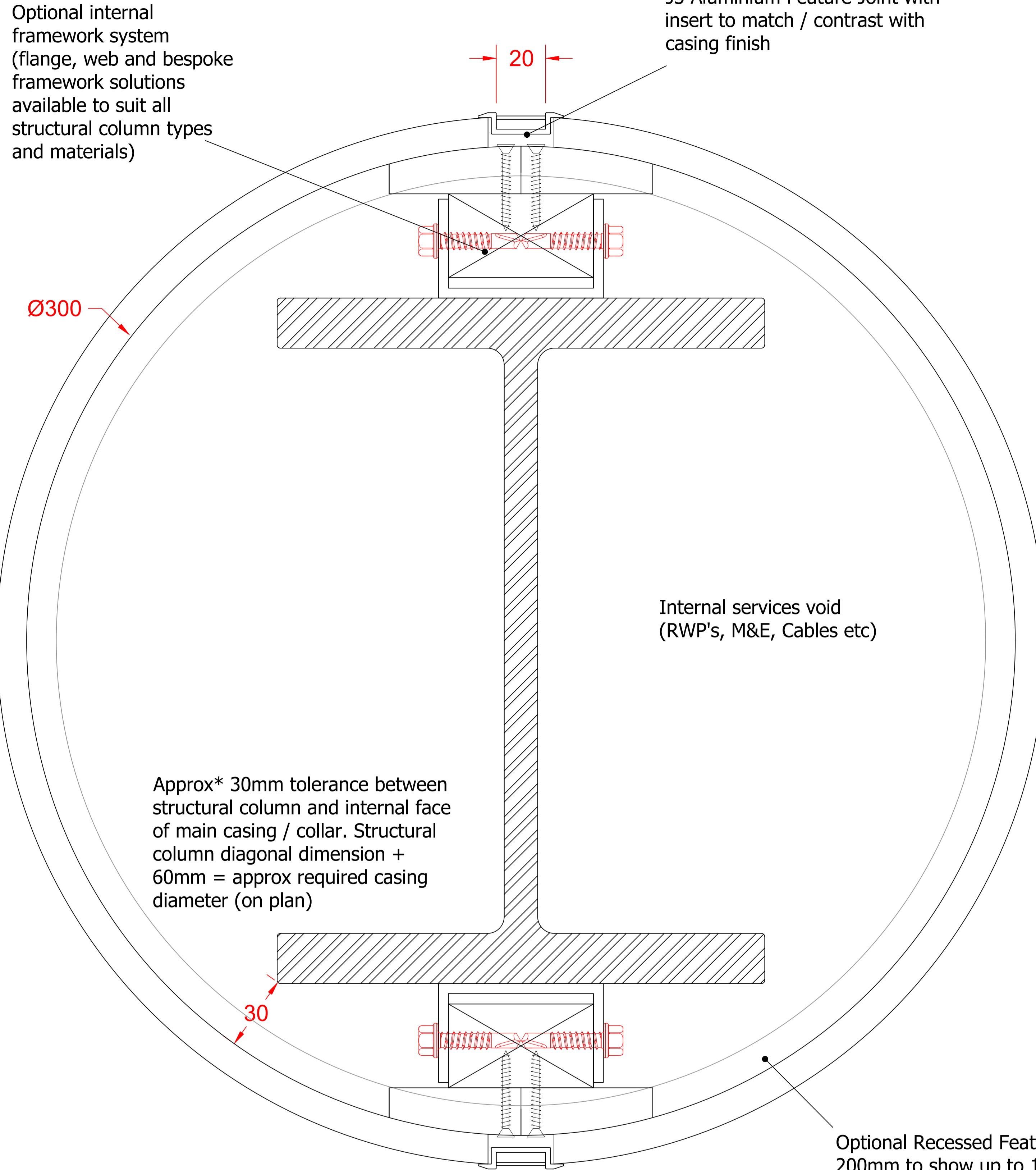
PLAN / SECTION A - A
