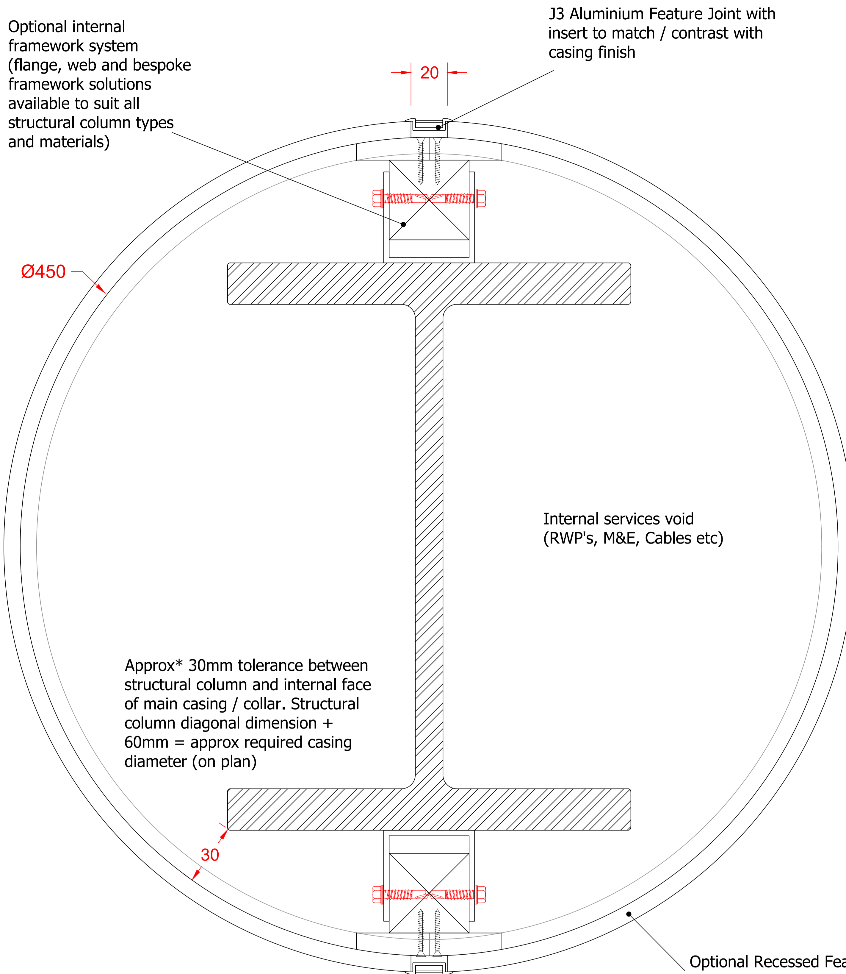
PLAN / SECTION A - A
