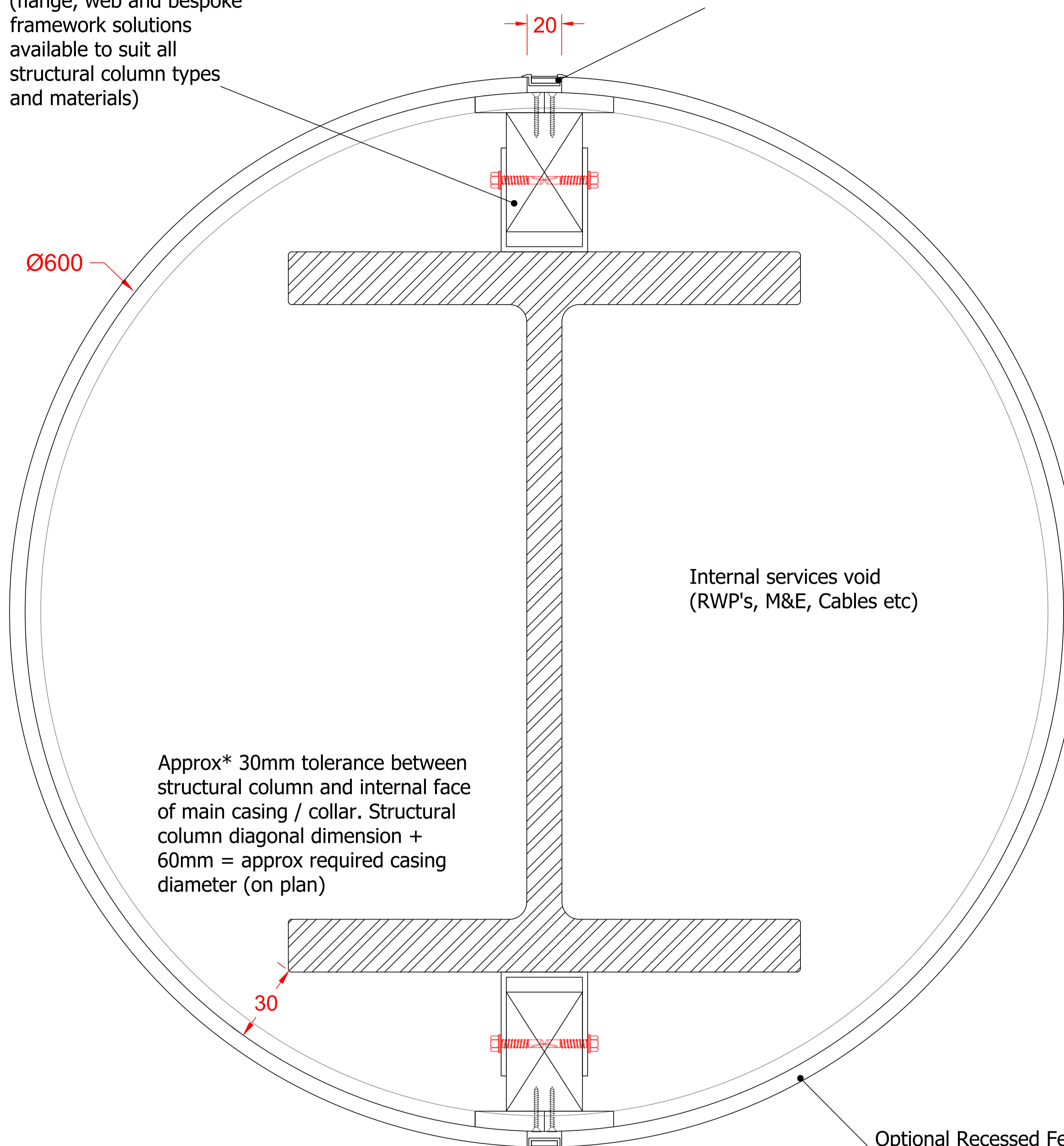
PLAN / SECTION A - A
