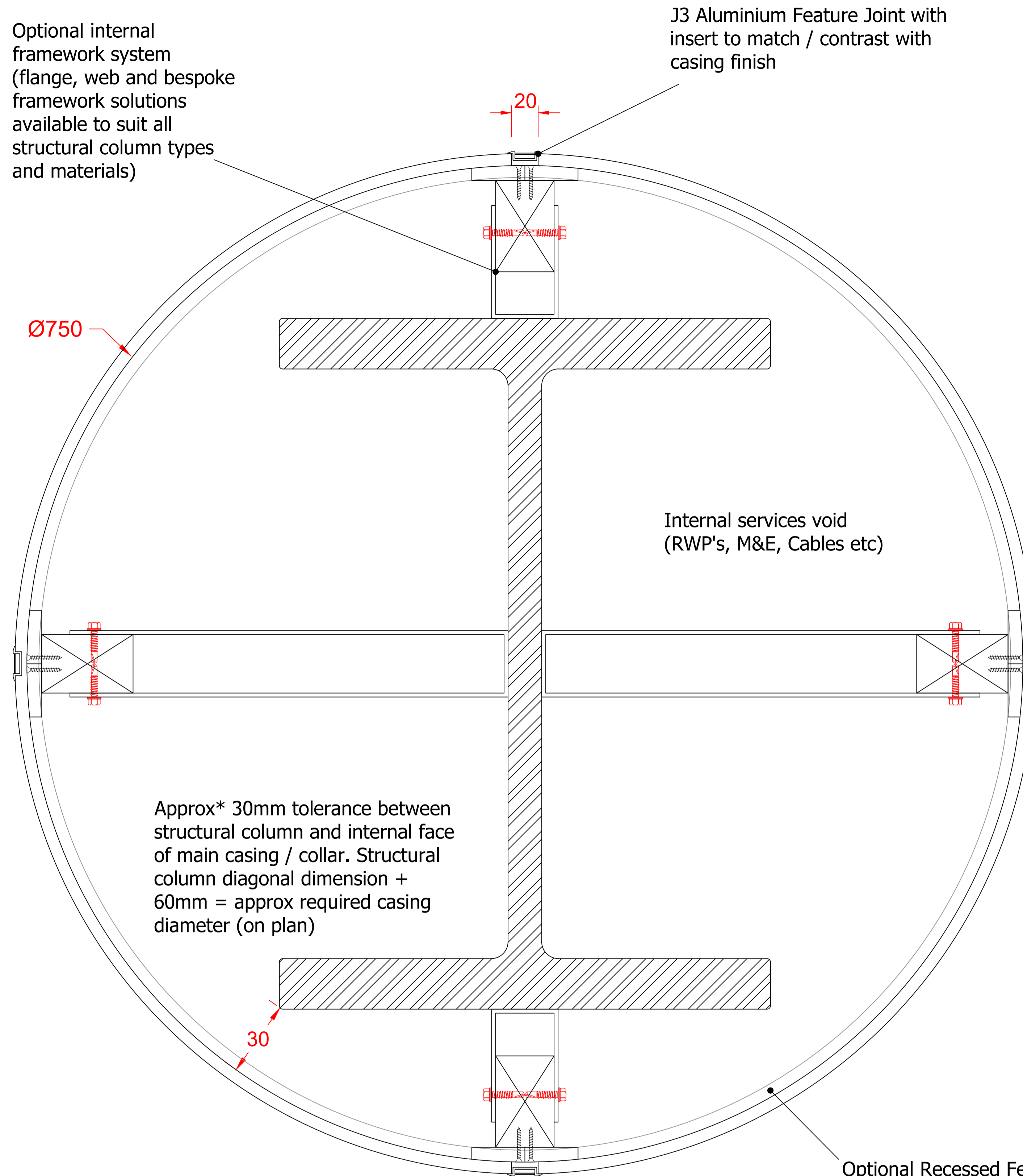
PLAN / SECTION A - A
