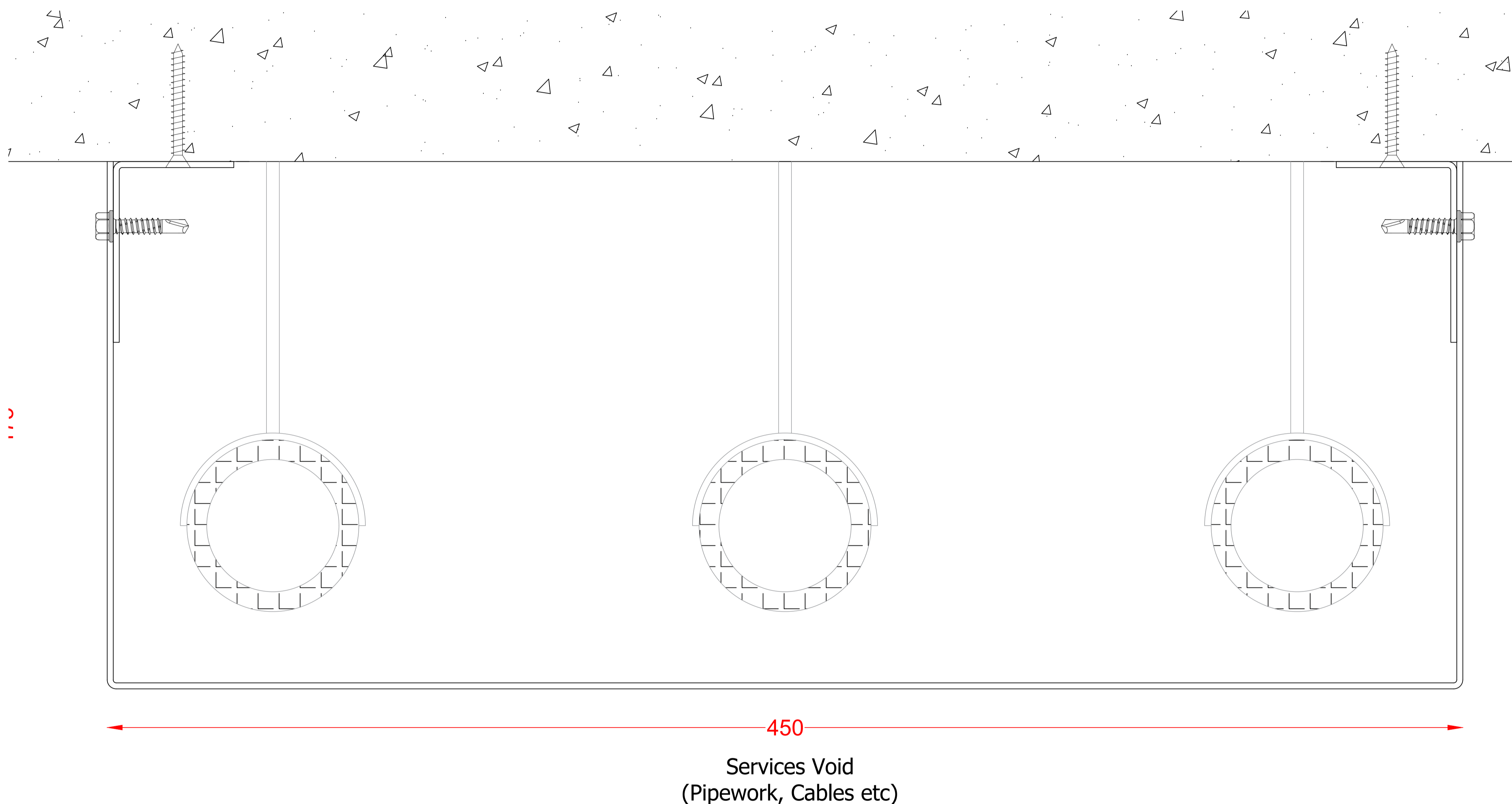
PLAN / SECTION DETAIL
