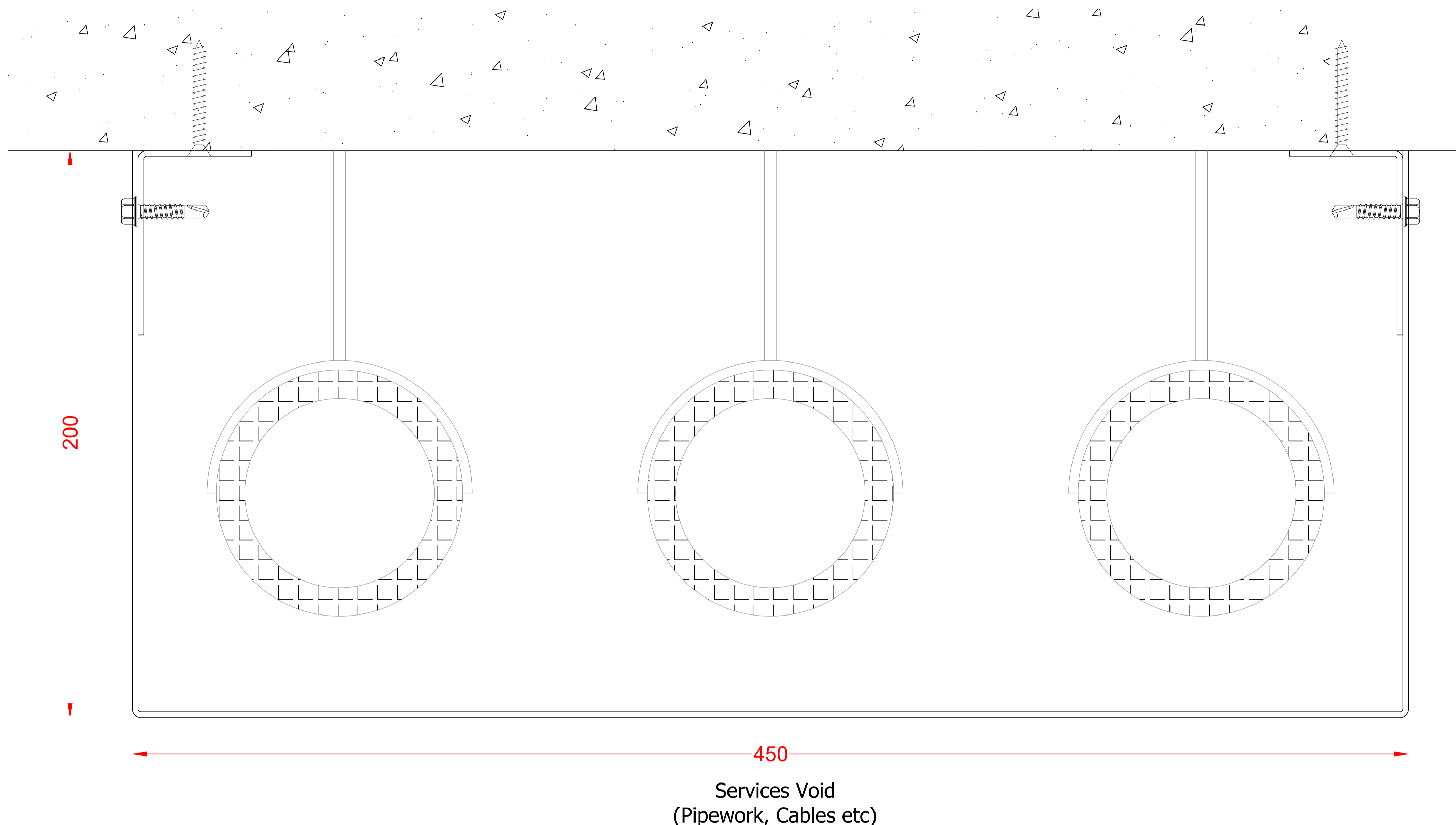
PLAN / SECTION DETAIL
