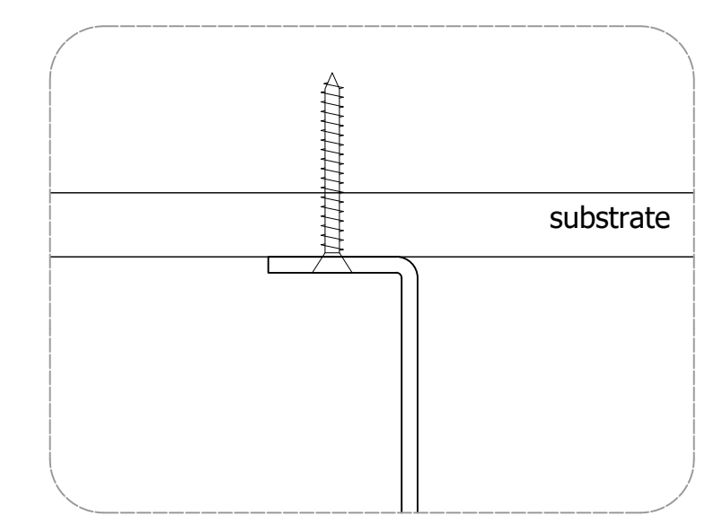
FIXING FLANGE OPTION
