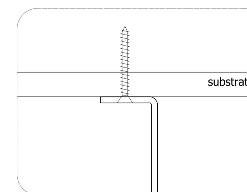
FIXING FLANGE OPTION
